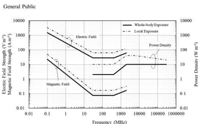
FIGURE 2. Reference levels for time averaged general public exposures of \geq 6 min, to electromagnetic fields from 100 kHz to 300 GHz (unperturbed rms values; see Tables 5 and 6 for full specifications).
